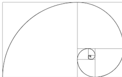
Gambar 2. 19 Fibonacci Numbers
