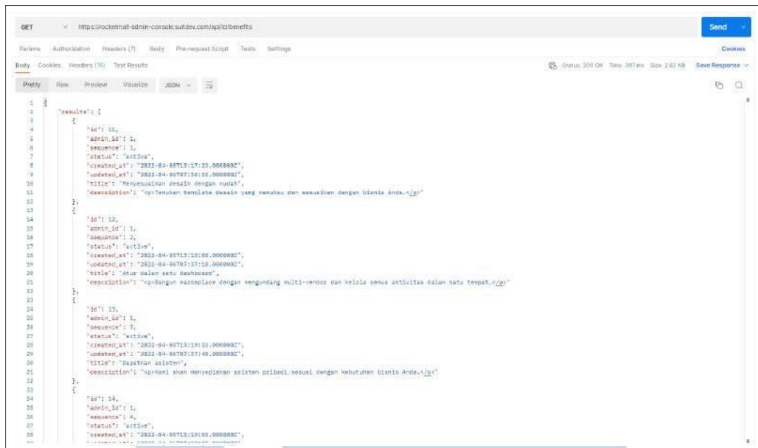
Gambar 3.16. API Benefits
