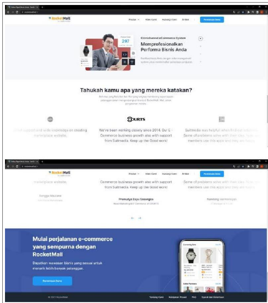
Gambar 3.25. Homepage Bagian 2
