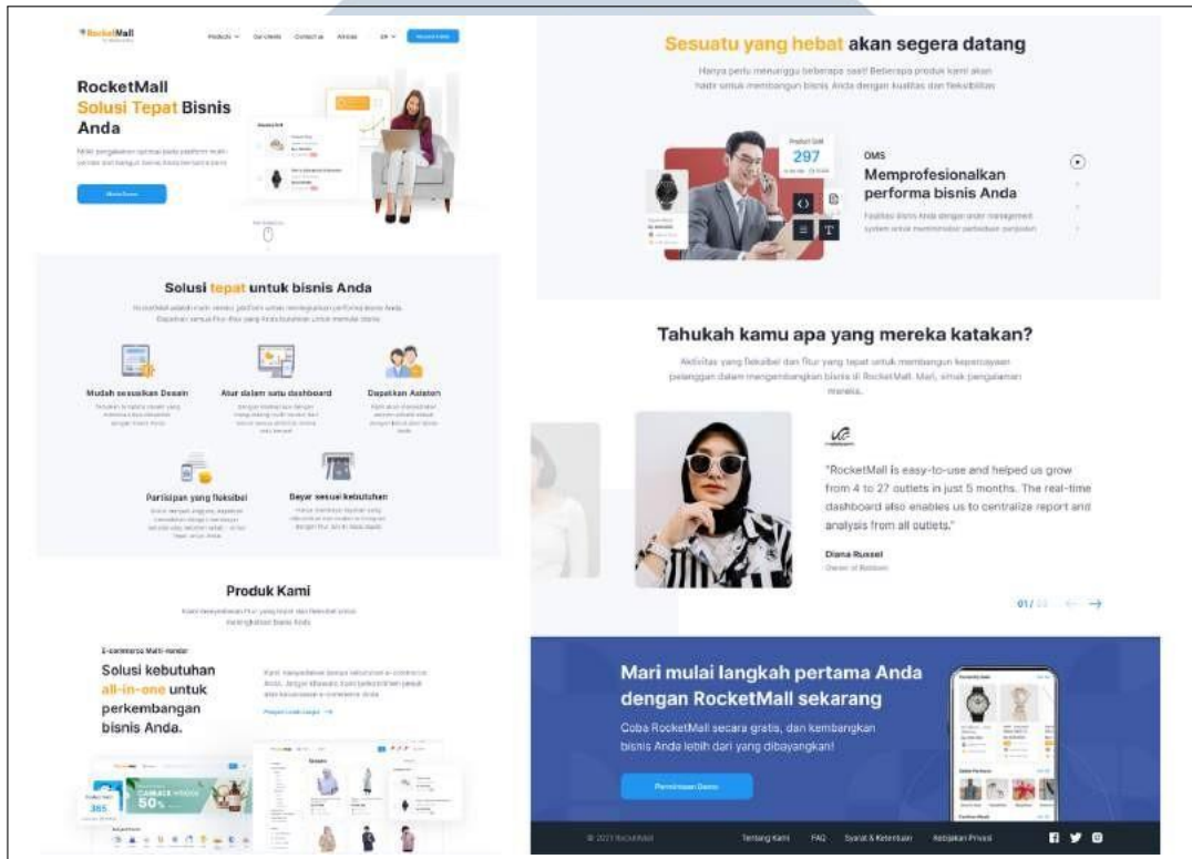
Gambar 3.3. Homepage
