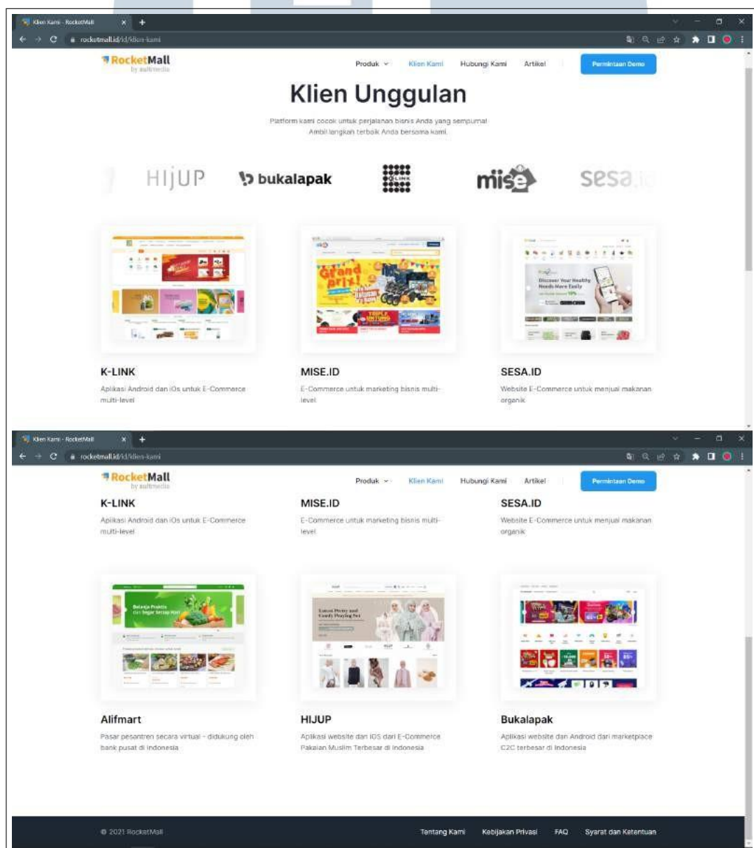
Gambar 3.27. Our Clients
