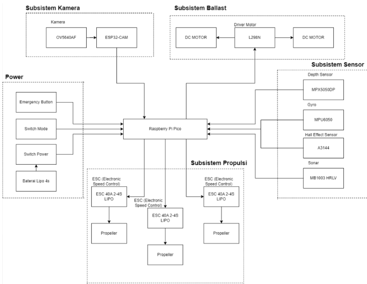
Gambar 25. Diagram Listrik Hydra
