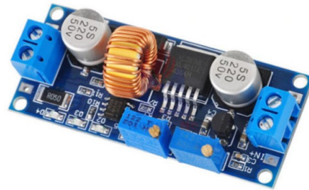
Gambar 22. Step Down Buck Converter 5A
