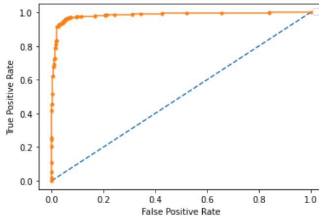
Figure 2: ROC AUC Plots of the Model Prediction
