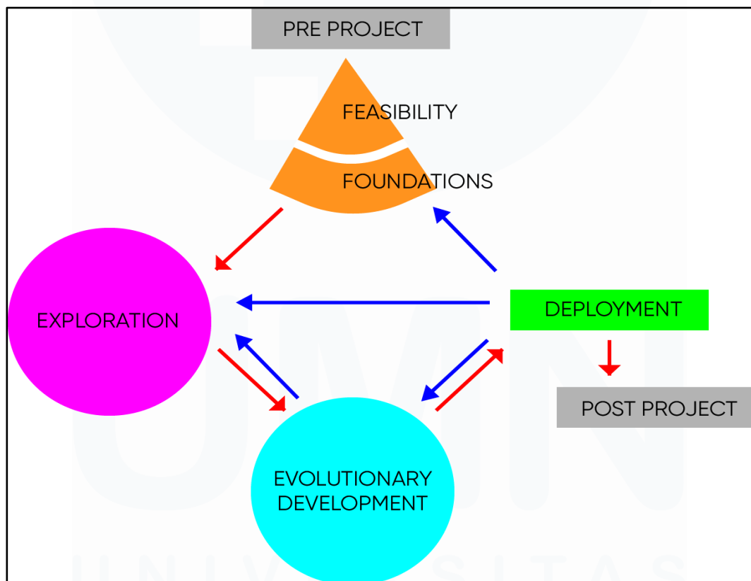
Gambar 3.1 Diagram DSDM
