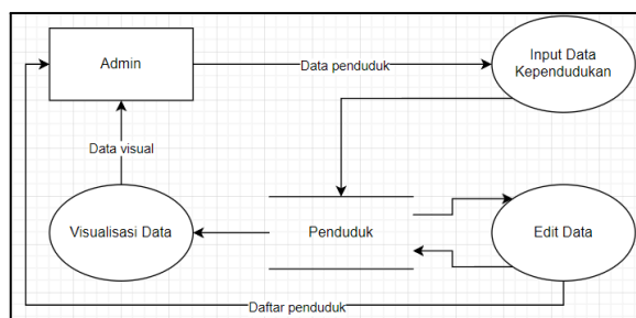
Gambar 3.3 DFD Level 1
