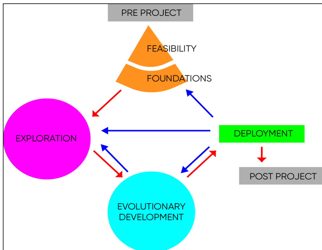
Gambar 3.1 Diagram DSDM
