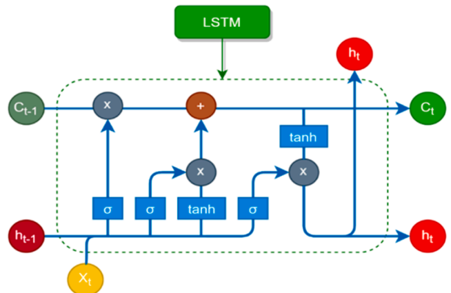
Fig. 3.2. LSTM architecture.
