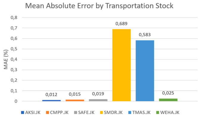
(b) Mean Absolute Error from Transportation Stock
