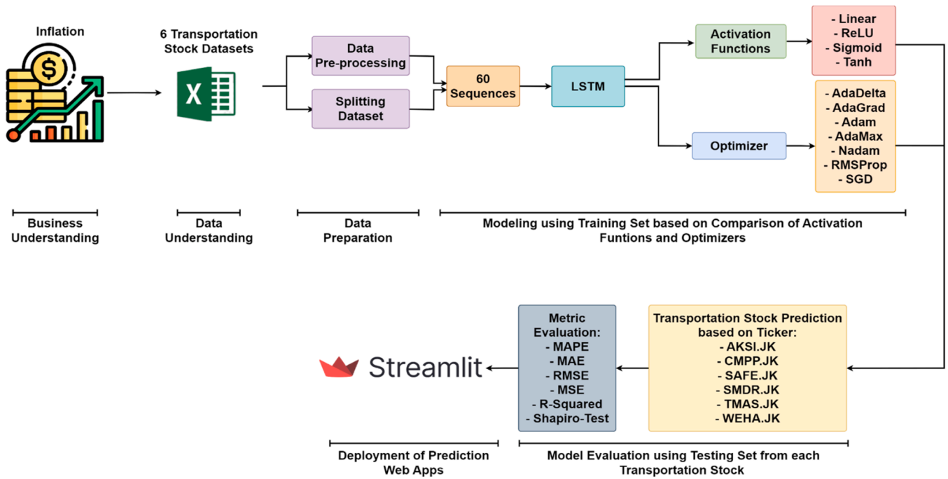
Fig. 3.1. Research workflow.
