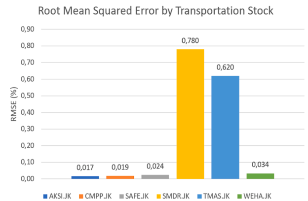
(f) Root Mean Squared Error from Transportation Stock
