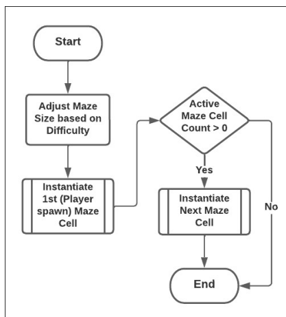
Figure 1: Maze Generation Flowchart
