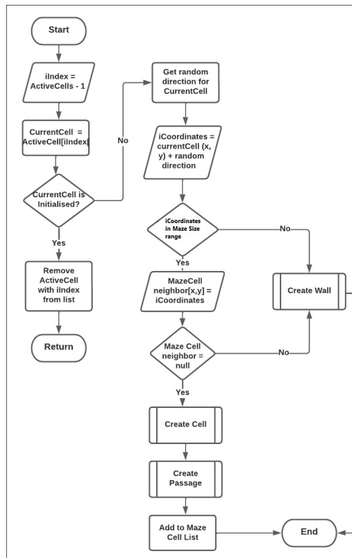
Figure 3: Maze Generation – Instantiate Maze Cells
