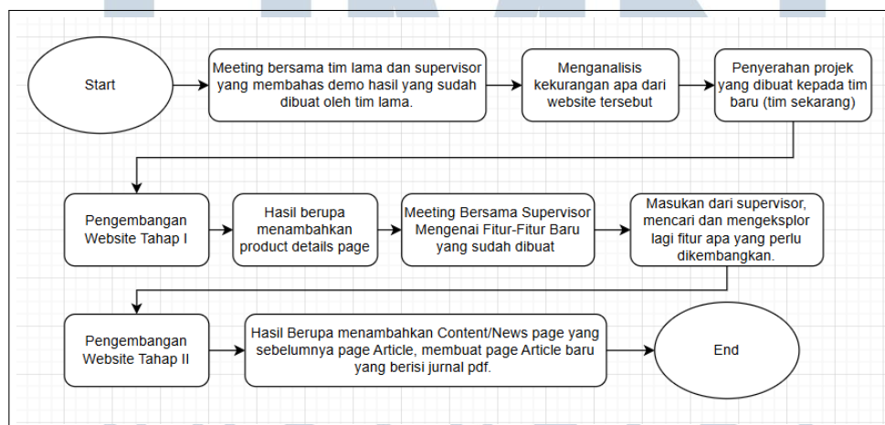
Gambar 3.3. Flowchart Pengembangan Website Official Baduy
