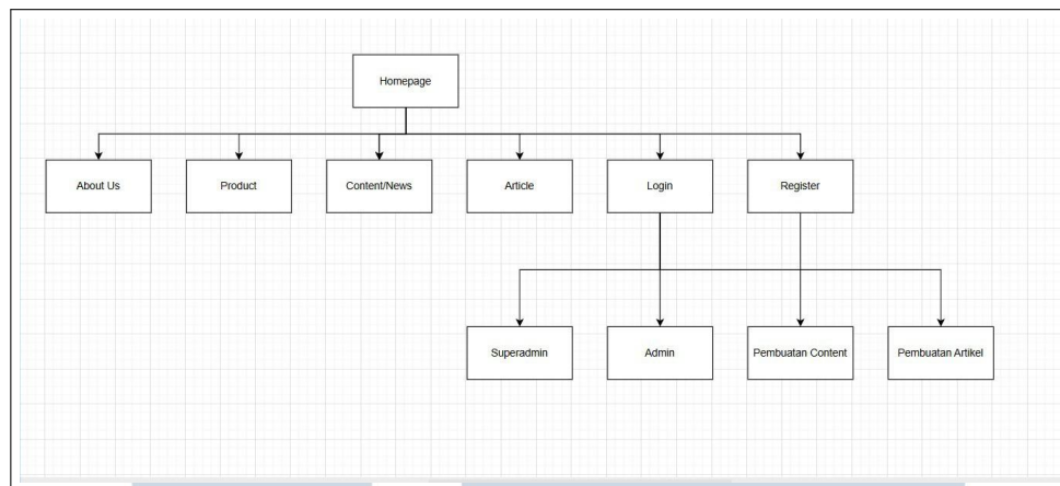
Gambar 3.2. Sitemap "Website Official Baduy"
