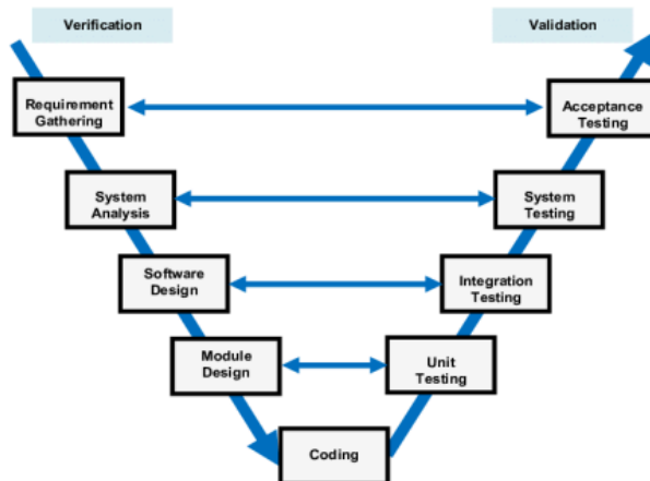
Gambar 2. V-Model
