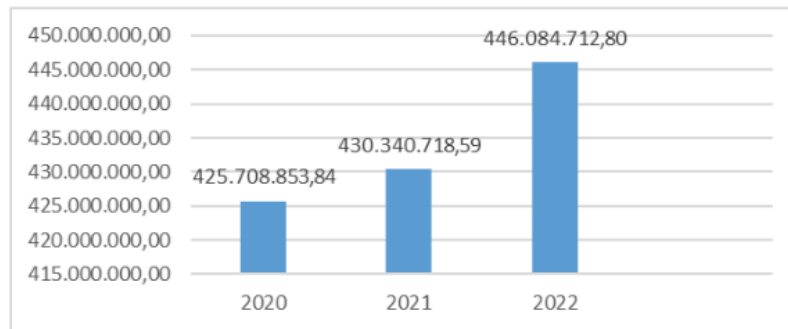
Figure 1 Outstanding Number of Corporate Bonds in 2020-2022 (in Millions of Rupiah) Source: OJK (2022)
