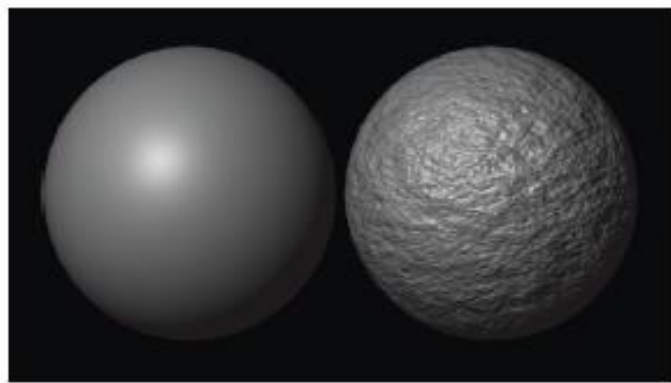
Gambar 2.8. Bump Material
