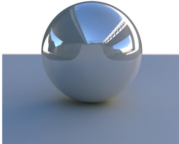
Gambar.2.4. Reflectivity
