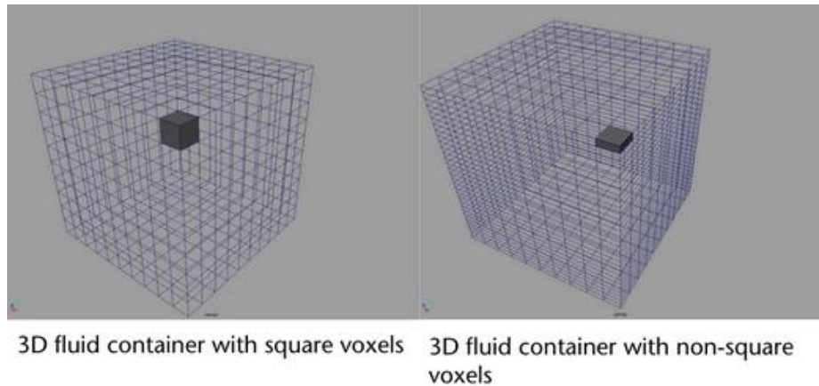
Gambar 2.11. 3D Container
