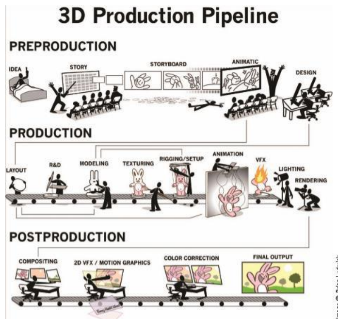
Gambar 2.1. Pipeline Animation
