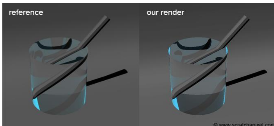
Gambar 2.5. Refraction
